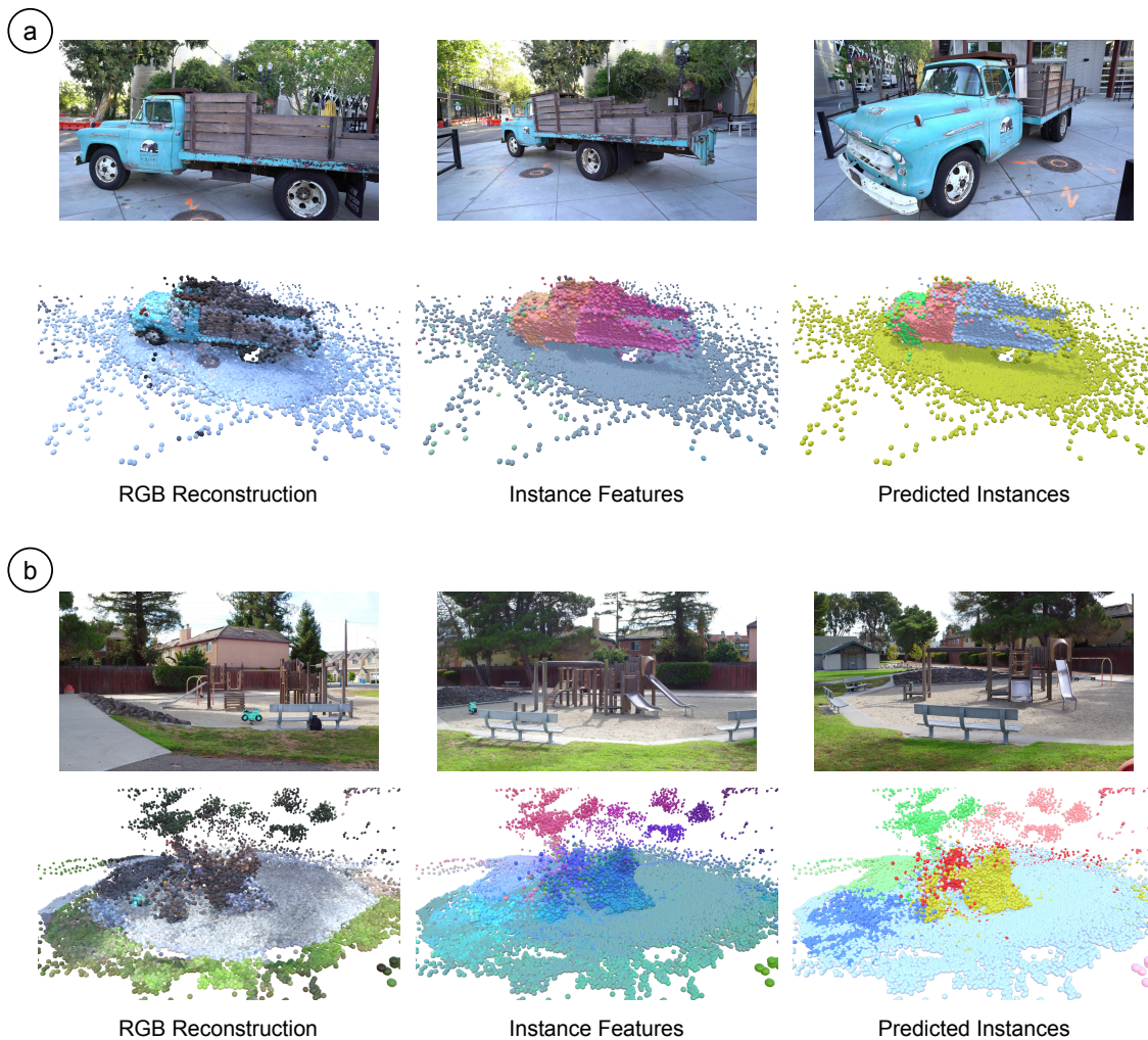
Figure 7: Outdoor generalization. UNITE trained on indoor scenes generalizes to outdoor scenes at small scales ③. At larger scales, domain shift in appearance as well as scene and object scales results in poor instance predictions ④.
